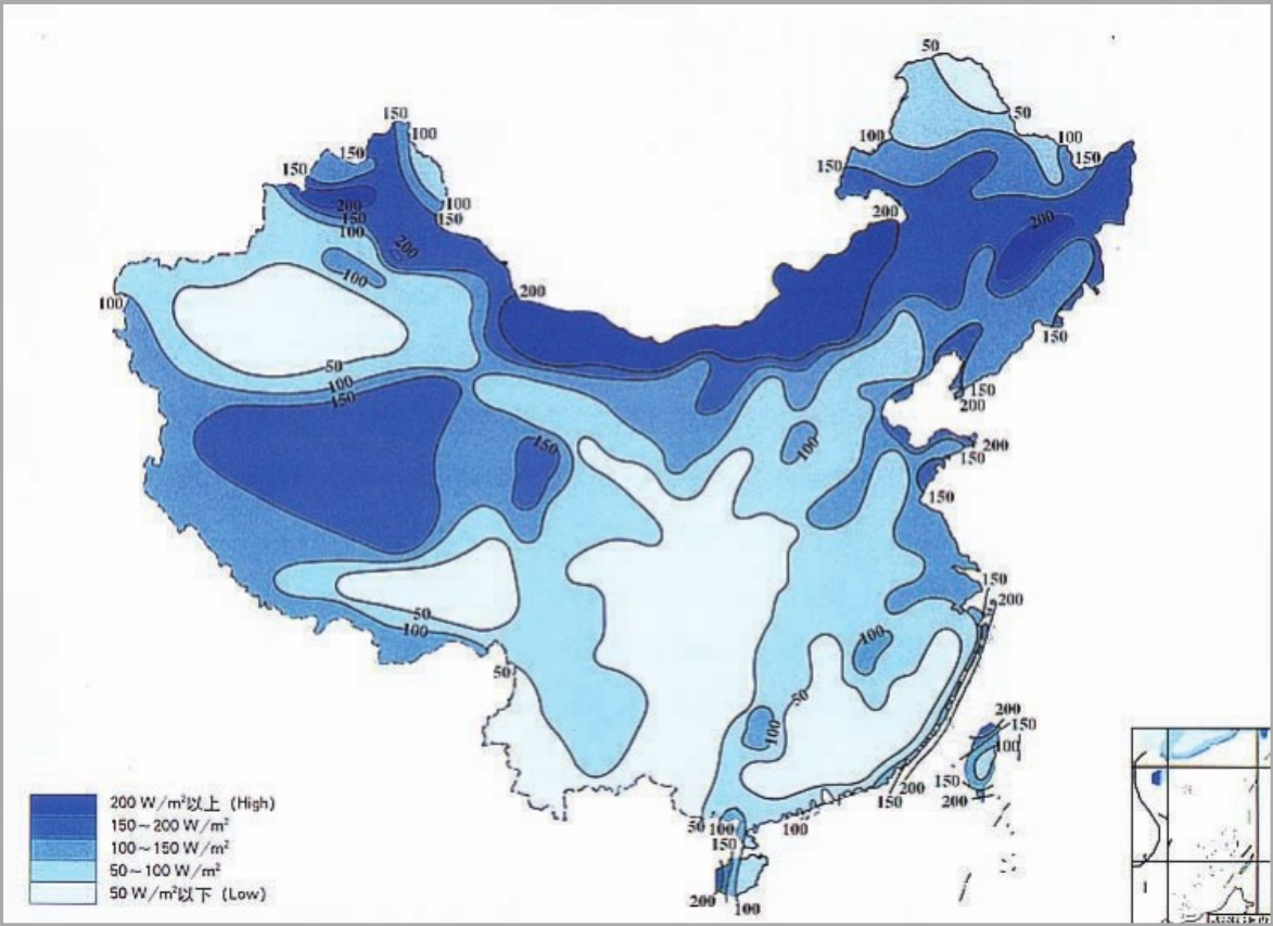
Annual distribution of wind energy resources in China
