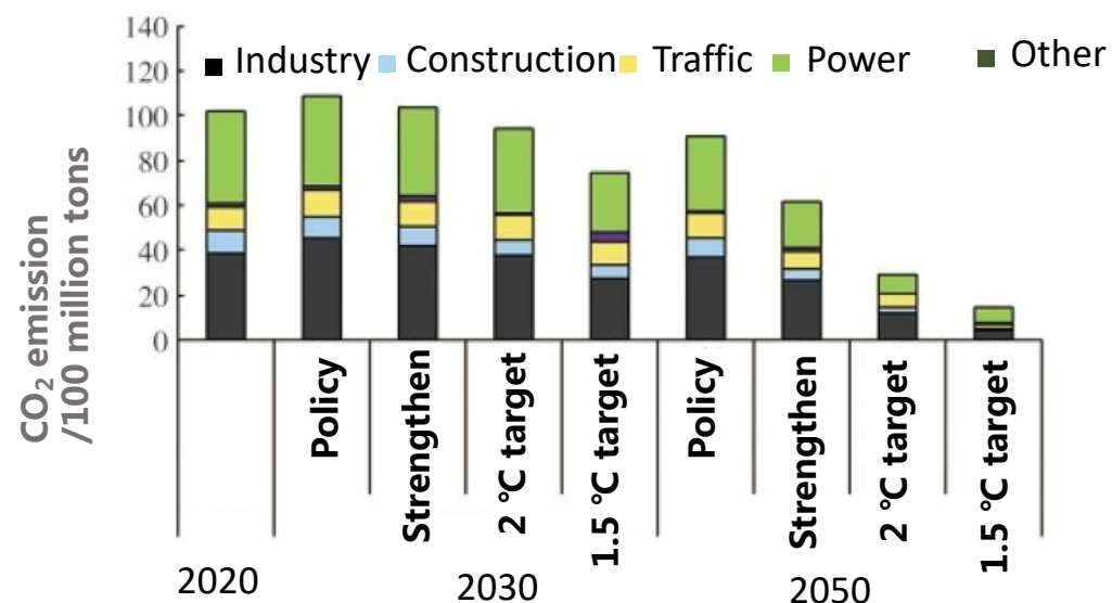
Composition of CO 2 emission by sector under different scenarios
