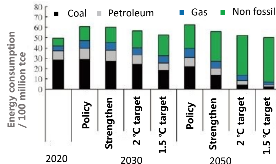
Composition of primary energy consumption in 2030 and 2050
