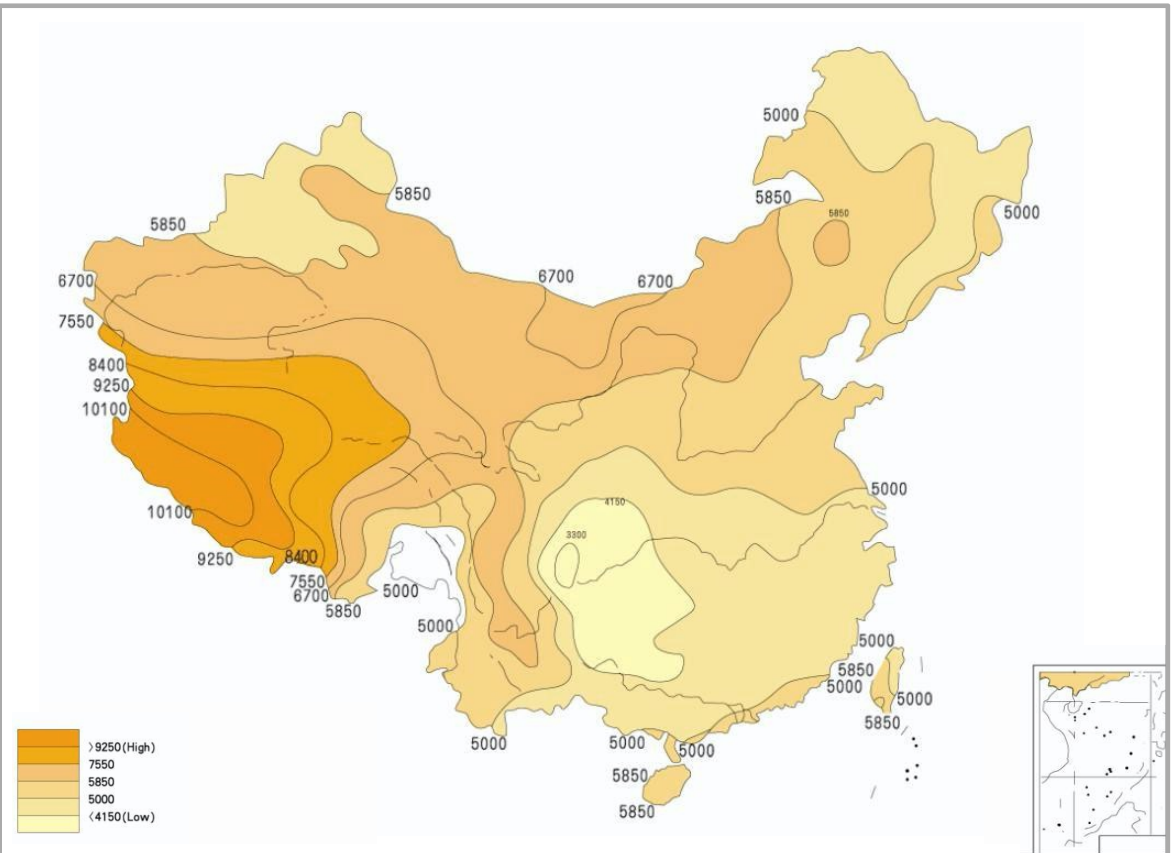
Annual distribution of solar energy resources in China
