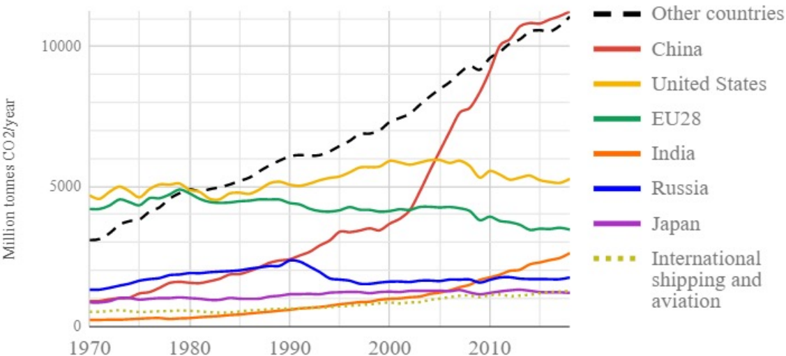
World fossil carbon dioxide emission 1970-2018
