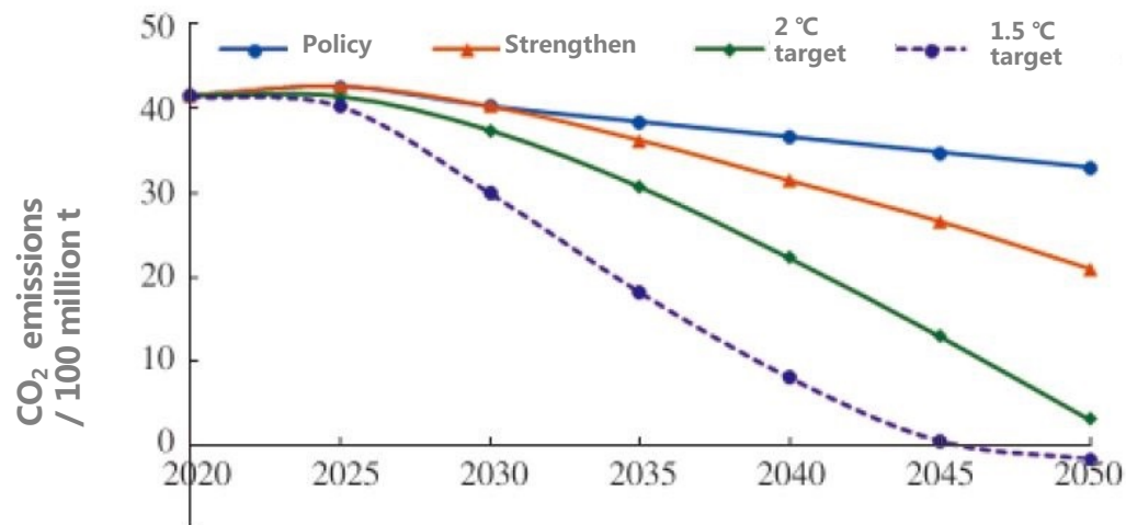
Carbon dioxide emissions from power sector under different scenarios (including CCS)
