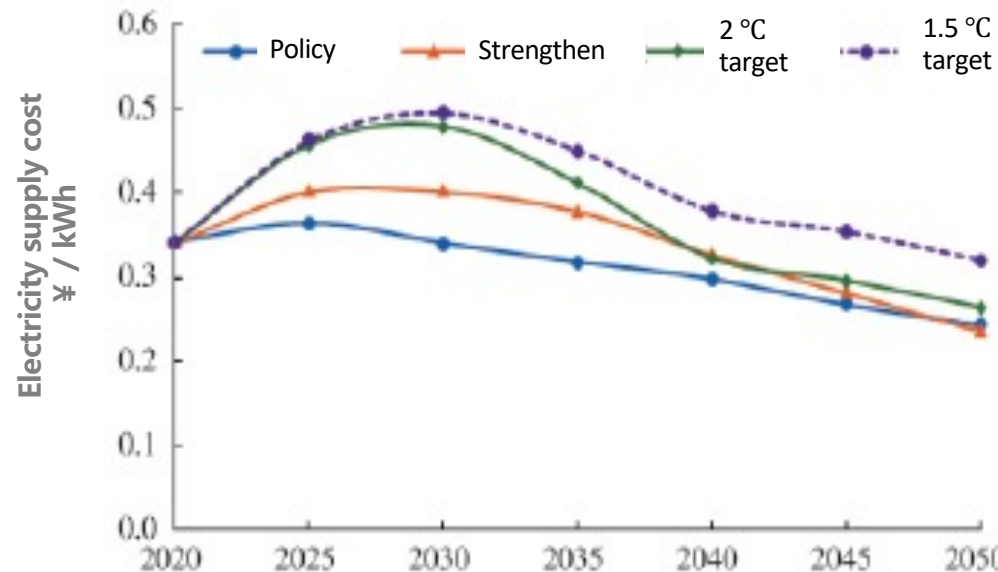
Trends of power supply costs under different scenarios
