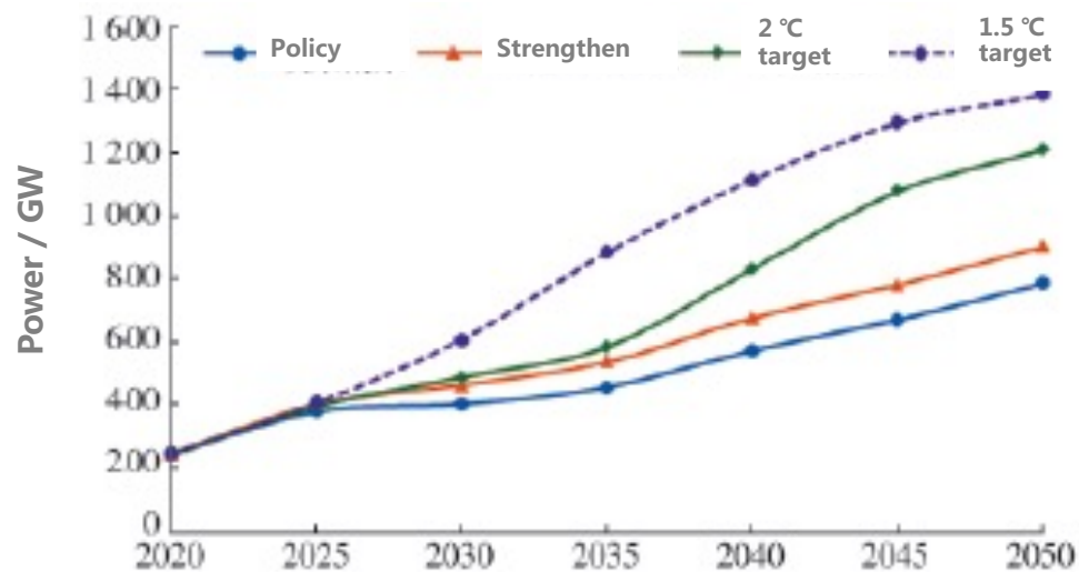
Total capacity of cross-regional power exchange under different scenarios
